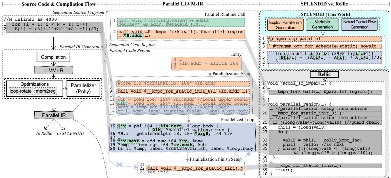
Figure 1: A comparison of code decompiled using Rellic [55] and SPLENDID. The motivating example is a simplified hot loop from jacobi-1d-imper in PolyBench [46]. The original sequential code is compiled into LLVM-IR, optimized by LLVM -O2, and parallelized using Polly [21]. The resulting parallel LLVM-IR then serves as the input for decompilation. Compared to code produced by Rellic, code produced by SPLENDID is portable to any host compiler and natural.
