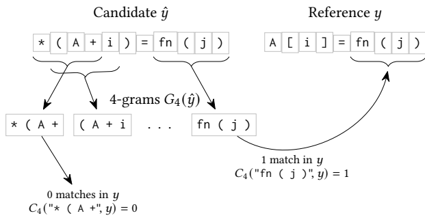
Figure 10: BLUE score calculation
